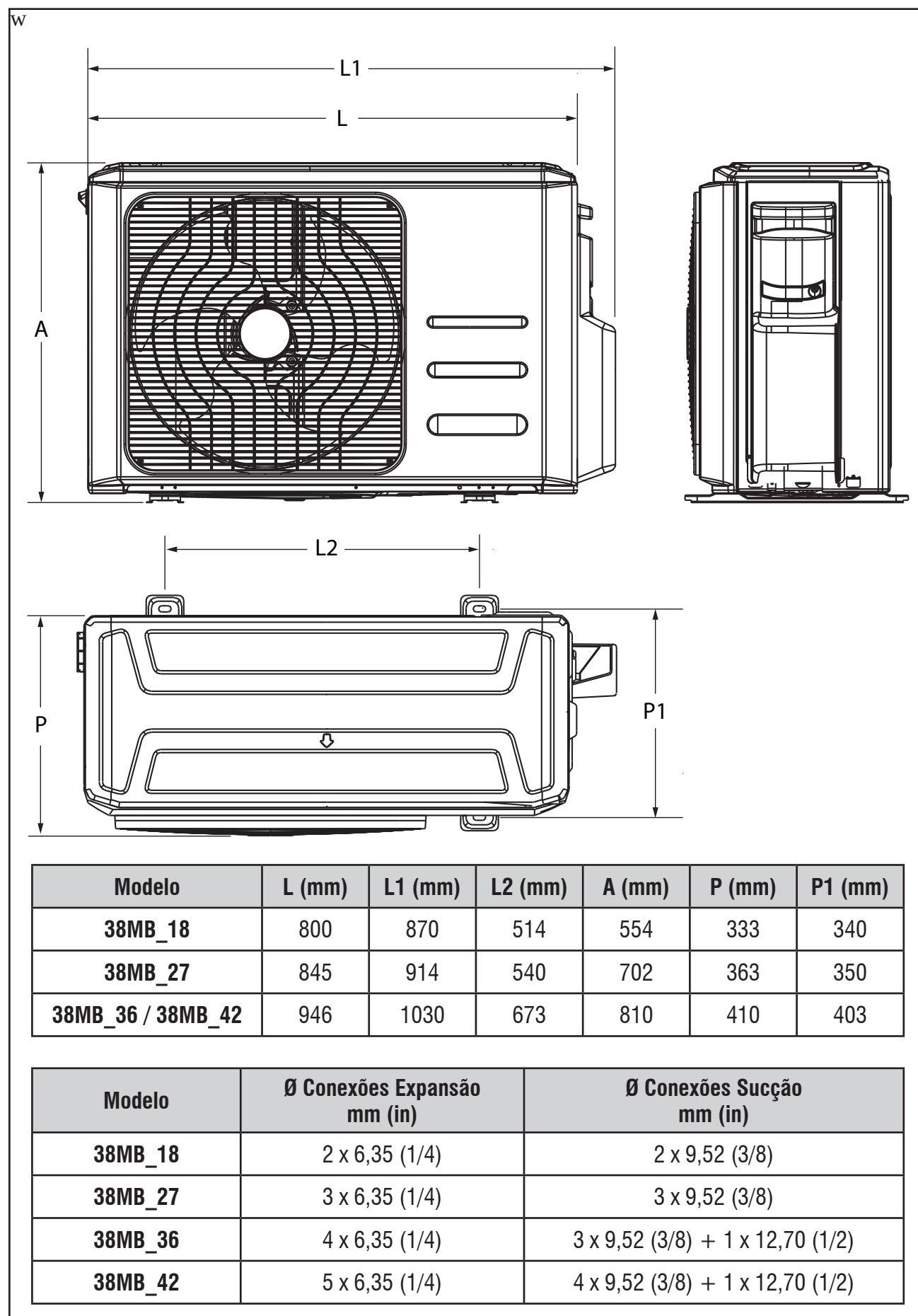
FIG. 5 - DIMENSIONAL
