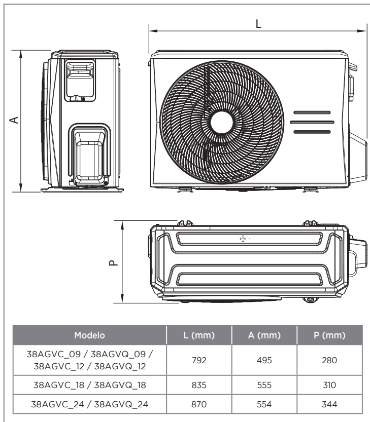
FIG. 4 - DIMENSIONAL
